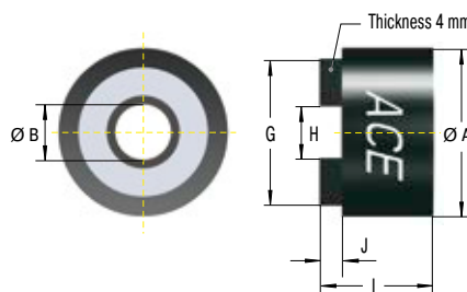
Standard Type
