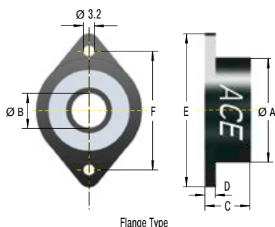
Flange Type
