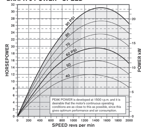
GRAPH 3 POWER - SPEED
