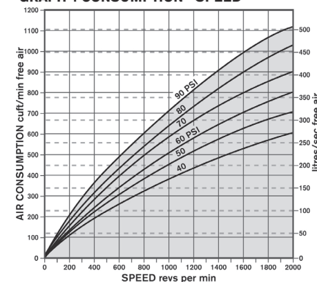
GRAPH 4 CONSUMPTION - SPEED
