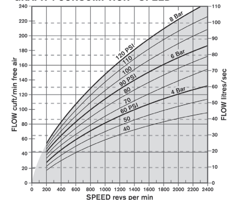
GRAPH 4 CONSUMPTION - SPEED
