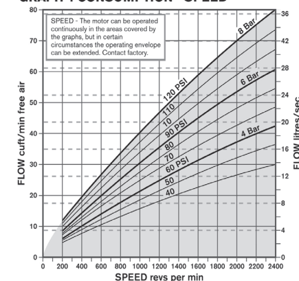
GRAPH 4 CONSUMPTION - SPEED
