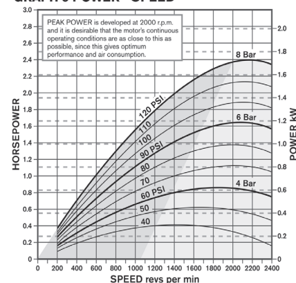
GRAPH 3 POWER - SPEED
